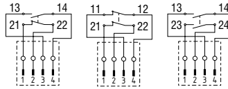
Connector Z/T 335, 336, 355
