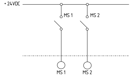
SLG 425I sensor connection
