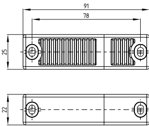
Actuator RST 36-1 / RST 36-1-R
