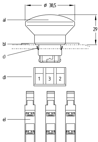
Fig. 28: a) EDRZ. emergency stop actuator; b) Emergency stop label; c) Clamping element; d) Mounting flange EFM; e) 3 × contact element EF
