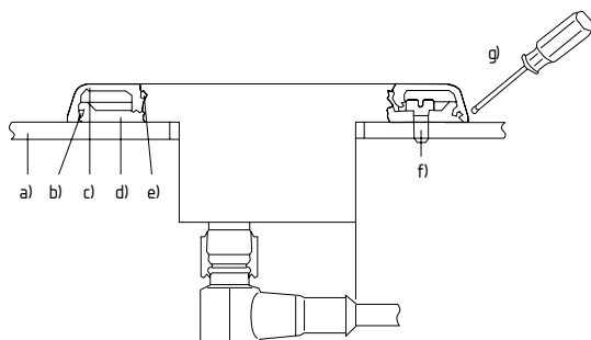
Fig. 8: a) Mounting surface; b) O-ring; c) Cover ring; d) Flat gasket; e) O-ring; f) 3 × fixing screws; g) Cover ring can be removed with screwdriver
