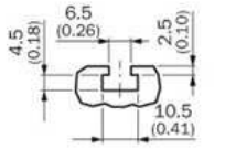
Sliding nut groove for side mounting
