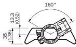
Mounting with swivel mount bracket (Part no. 2019659)
