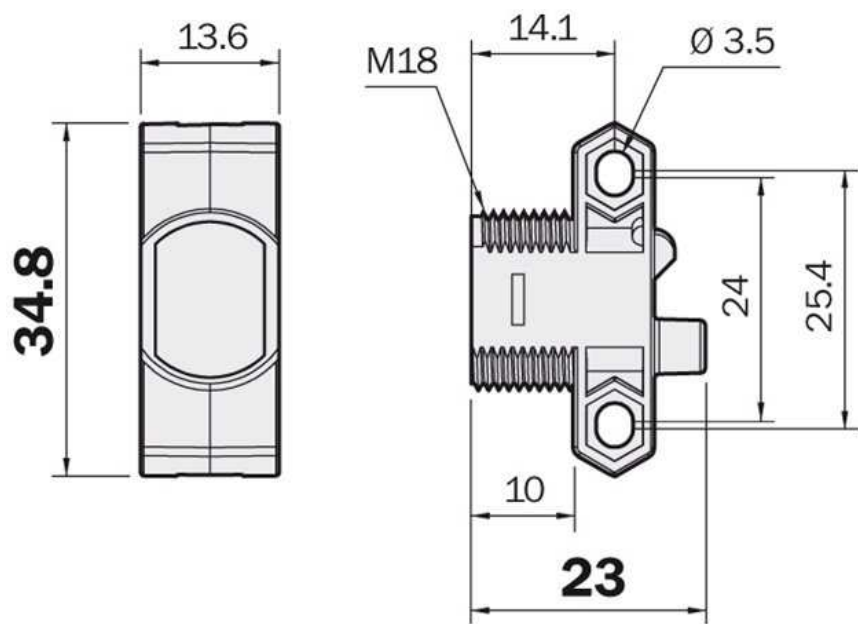
Dimensional drawing
