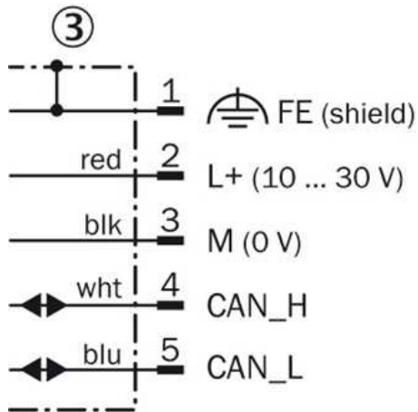
M12 (A-coded)
