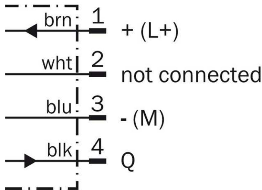
Connection diagram
