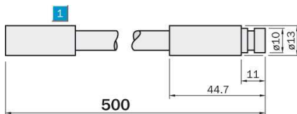
1 LLUV 5, Fibre-optic cable, mind. bend radius R_{min} = 60 mm
